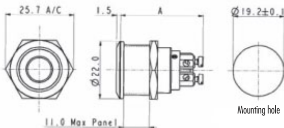
DIMENSION A: 31.0 MM - 32.7 MM DEPENDING ON TERMINAL
